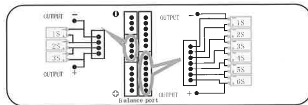
Balance port and Individual Cell connection diagram
