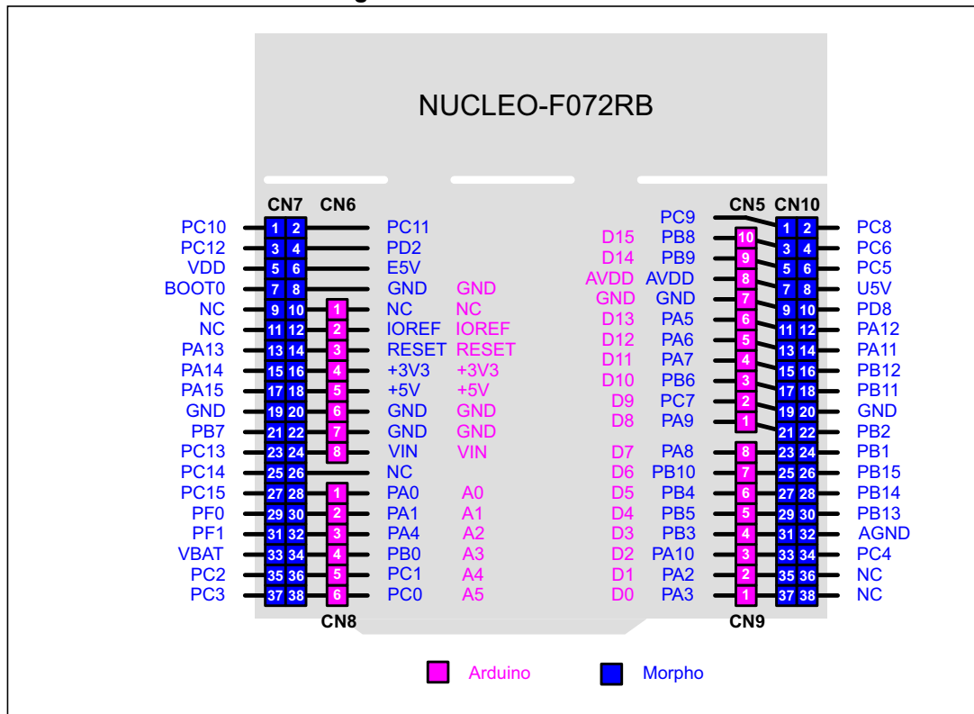
Figure 13. NUCLEO-F072RB
